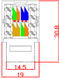
Cat.6 Keystone
