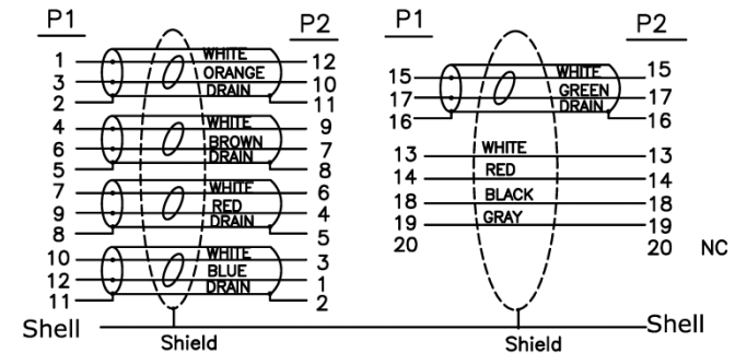
Pin Assignment
