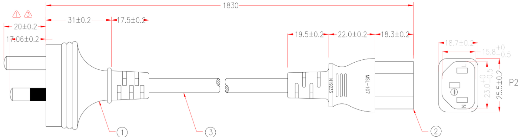
PLUG: MSL-301
