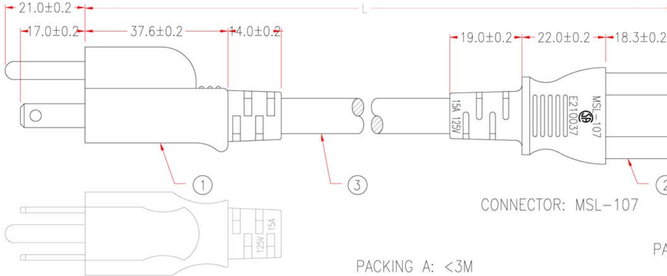
PLUG: MSL-105
