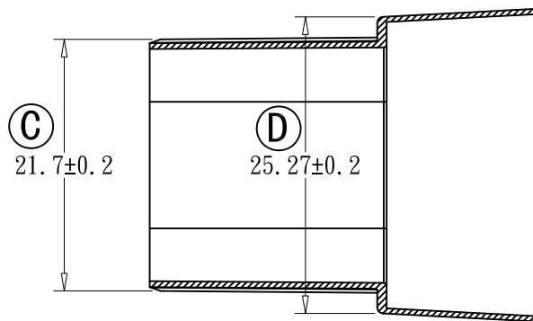
VIEW: A-A
